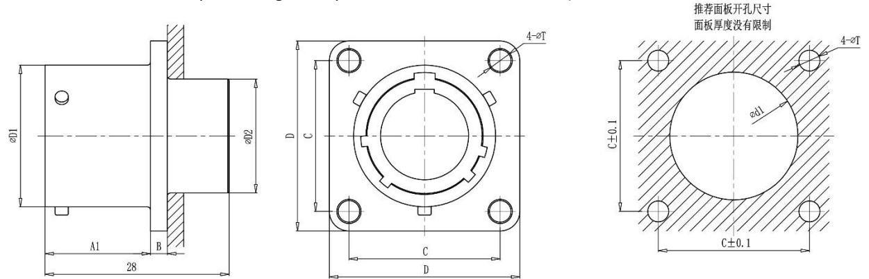
MS27496 Box Mount Square Flange Receptacle ( Front Panel Mounted)
