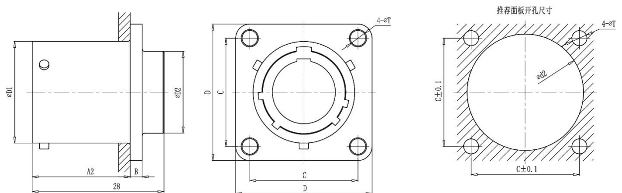
MS27505 Box Mount Square Flange Receptacle ( Back Panel Mounted)
